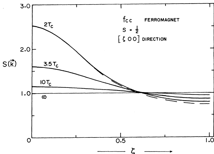
FIG. 2. Neutron scattering S(\mathbf{k}) at high temperatures from a face-centered cubic ferromagnet with spin \frac{1}{2} . The scattering is plotted from the origin to the [100] zone boundary. As the temperature approaches the ordering temperature T_c , the scattering becomes peaked about the origin. The dashed line shows the analogous plot for \chi(\mathbf{k}) at temperature 2T_c ; it should be within the scope of current neutron scattering techniques to observe the differences between \chi(\mathbf{k}) and S(\mathbf{k}) .
