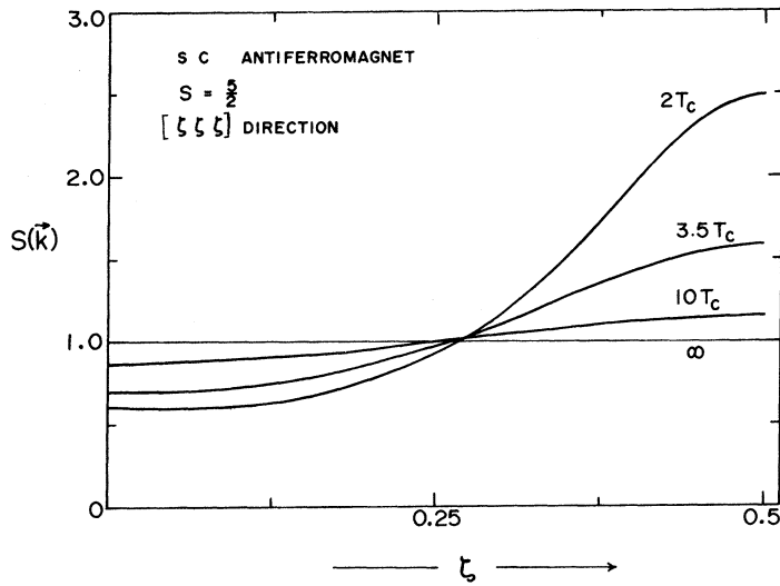
FIG. 1. Neutron scattering S(\mathbf{k}) at high temperatures for a simple-cubic antiferromagnet with spin \frac{5}{2} plotted from the origin (0, 0, 0) to the antiferromagnetic reciprocal-lattice vector (\frac{1}{2}, \frac{1}{2}, \frac{1}{2}) . The scale is such that for a non-interacting spin system S(\mathbf{k}) = 1 . As the temperature approaches the ordering temperature T_N the scattering becomes peaked about the point (\frac{1}{2}, \frac{1}{2}, \frac{1}{2}) .
